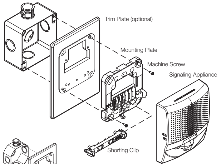
Double Gang Electrical Box
