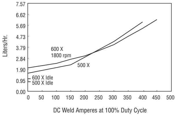
Fuel Consumption Curve
