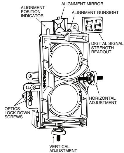
FIGURE 12. COARSE ALIGNMENT PROCEDURE:
