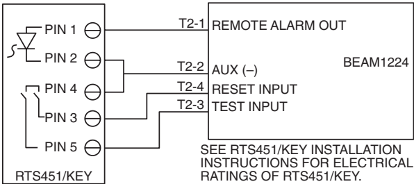
FIGURE 8. WIRING DIAGRAM (RTS451):
