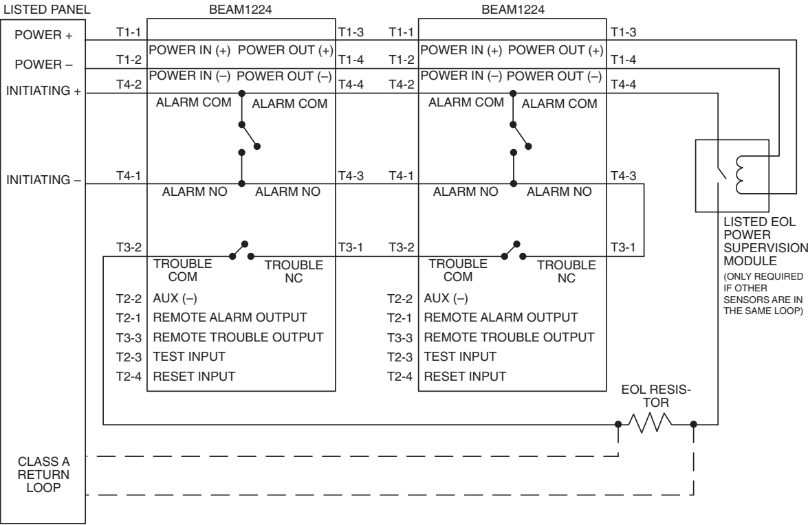
FIGURE 7. WIRING CONNECTIONS AT DETECTOR:
