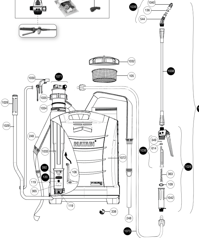
1 M ALUMINIUM LANCE TUBE WITH COMPLETE ELBOW Reference 8.34.60.871 1.5 M ALUMINIUM LANCE TUBE WITH COMPLETE ELBOW Reference 8.34.60.872
